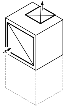
FRONT/RIGHT VIEW REVERSE EVAPORATOR FRONT RETURN TOP DISCHARGE (CATALOG OPTION) ②
